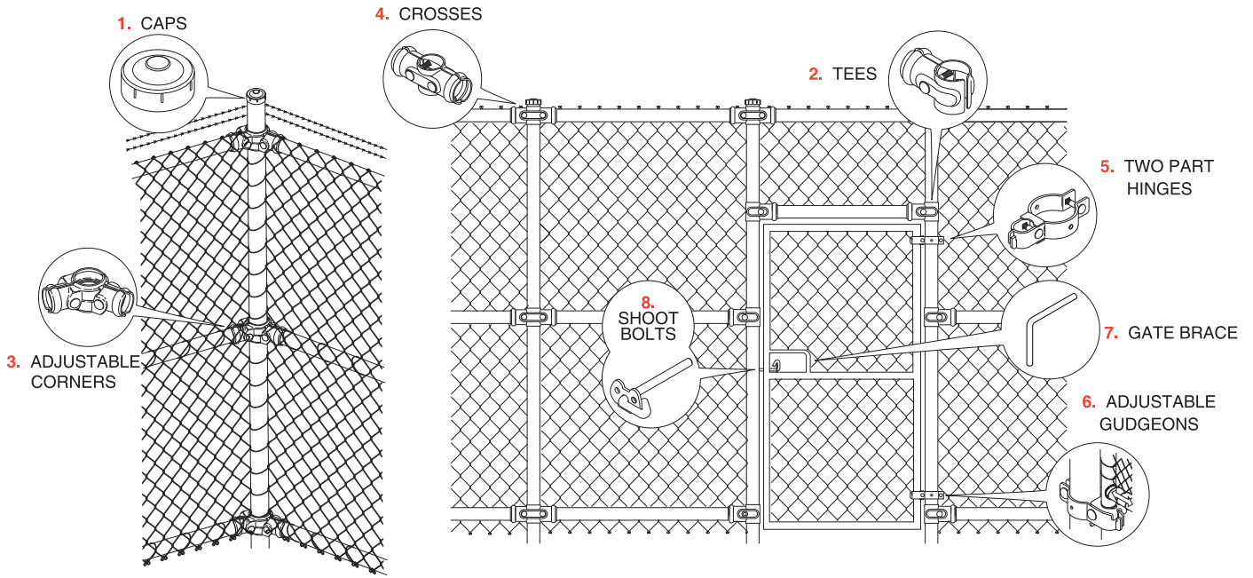
1 - CAPS GALVANISED
